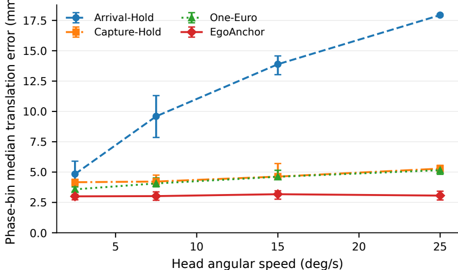
Capture-time semantics limit rotation-induced world error
