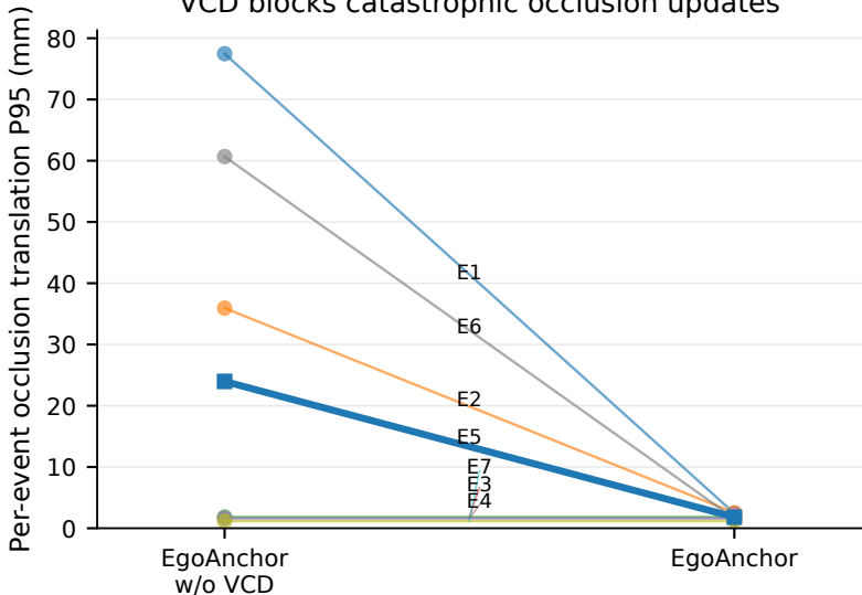
VCD blocks catastrophic occlusion updates
