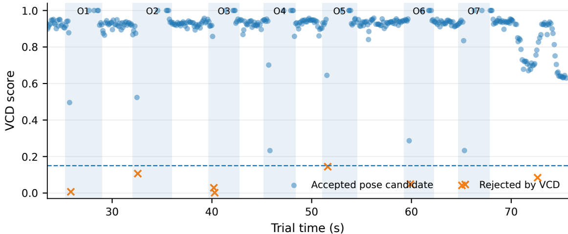
VCD decisions and occlusion intervals
