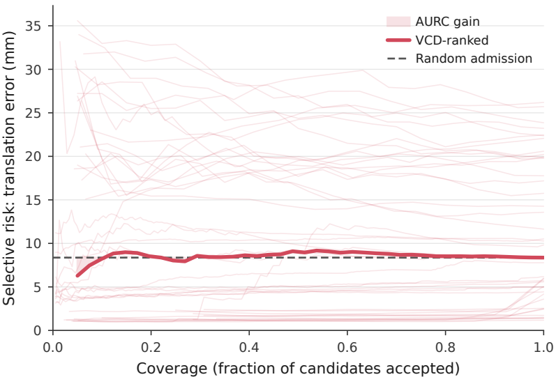
VCD risk-coverage (full EgoAnchor)
