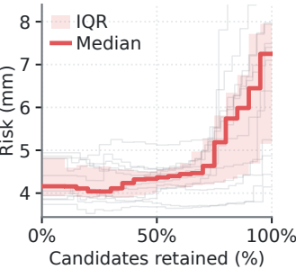
(c) VCD risk-coverage
