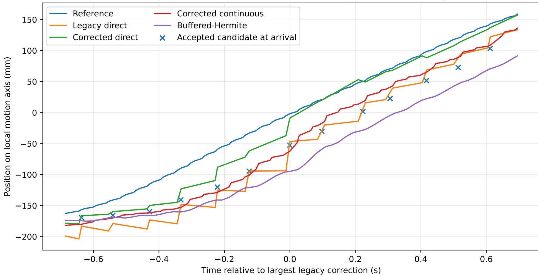
Real log: asynchronous correction discontinuity and corrected output
