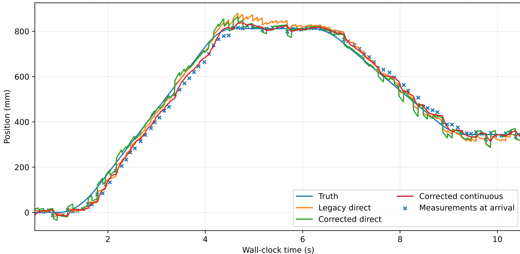
Synthetic causal test: 10 Hz measurements, 170 ms arrival delay, 90 Hz rendering
