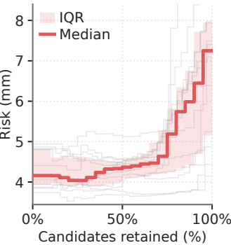
(c) VCD risk-coverage
