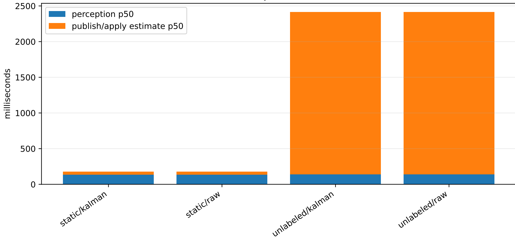
Latency Breakdown
