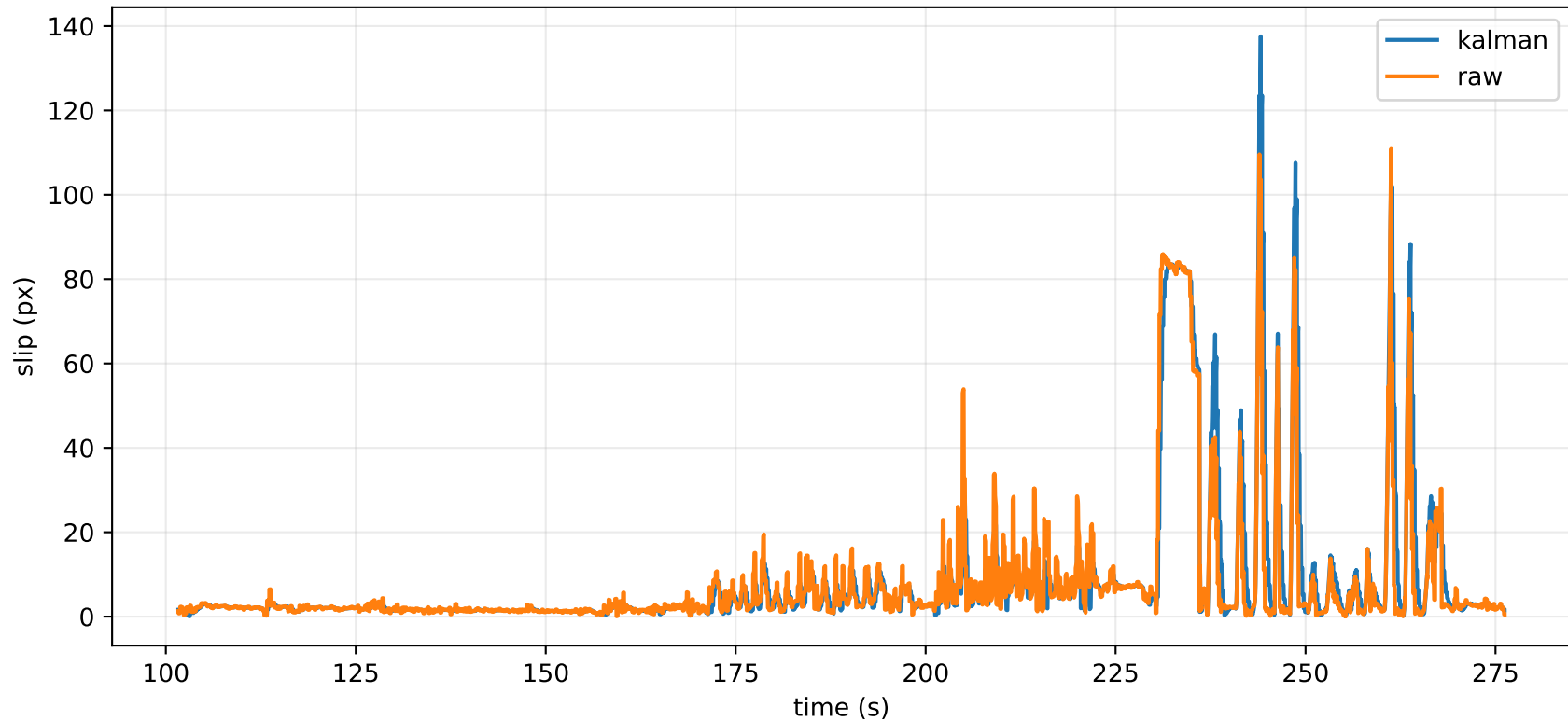
Screen-Space Slip
