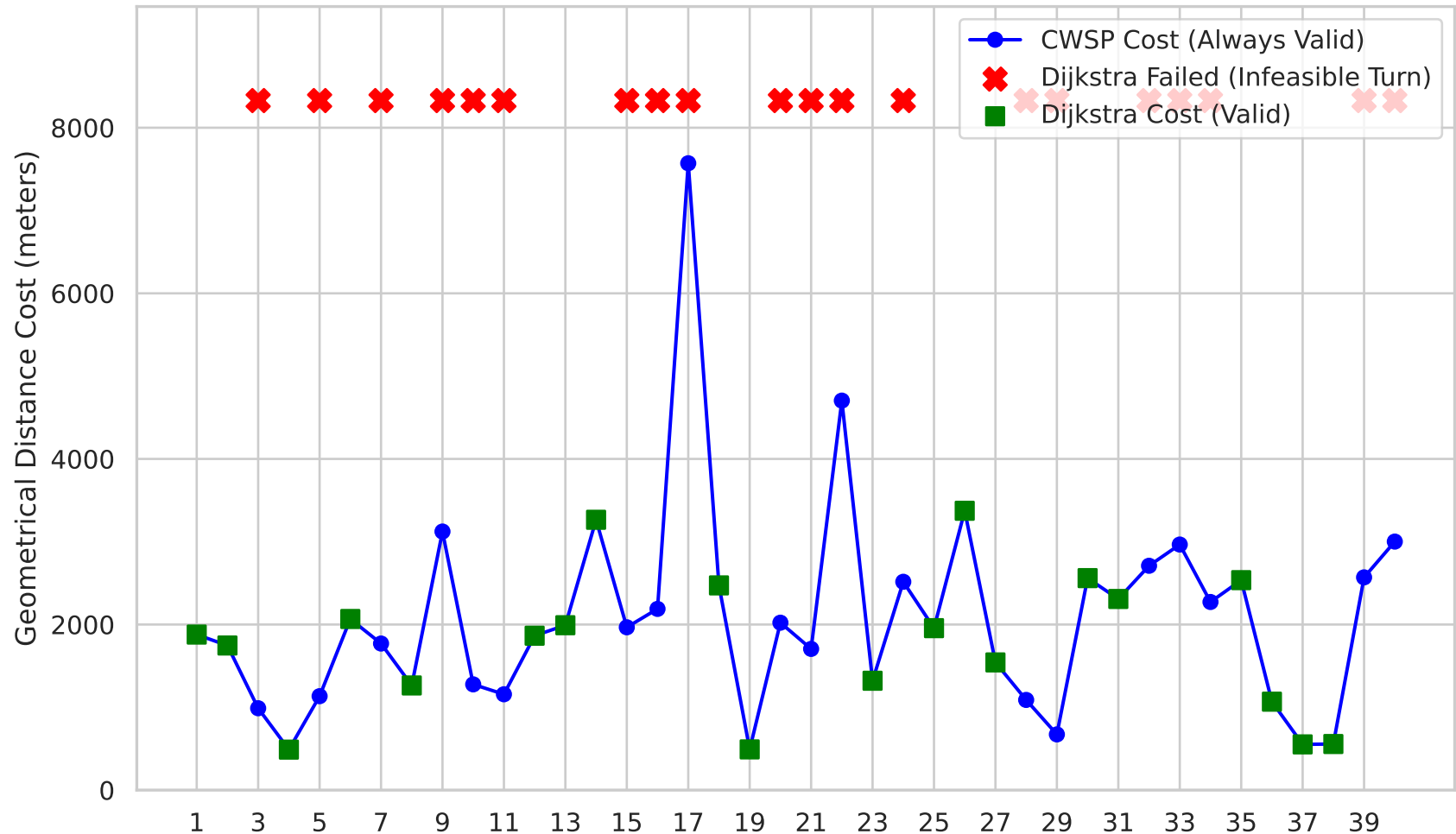
Path Cost Comparison: CWSP vs Traditional Dijkstra
