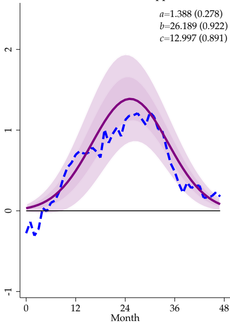
Gaussian Basis Function Approximation
