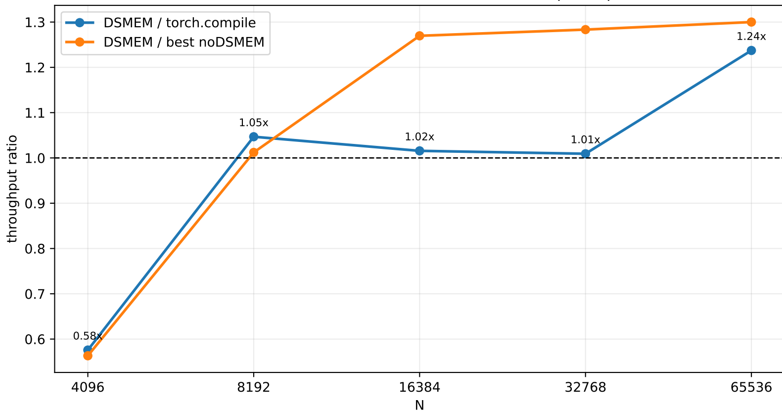
Row-wise Affine Standardization DSMEM Speedup
