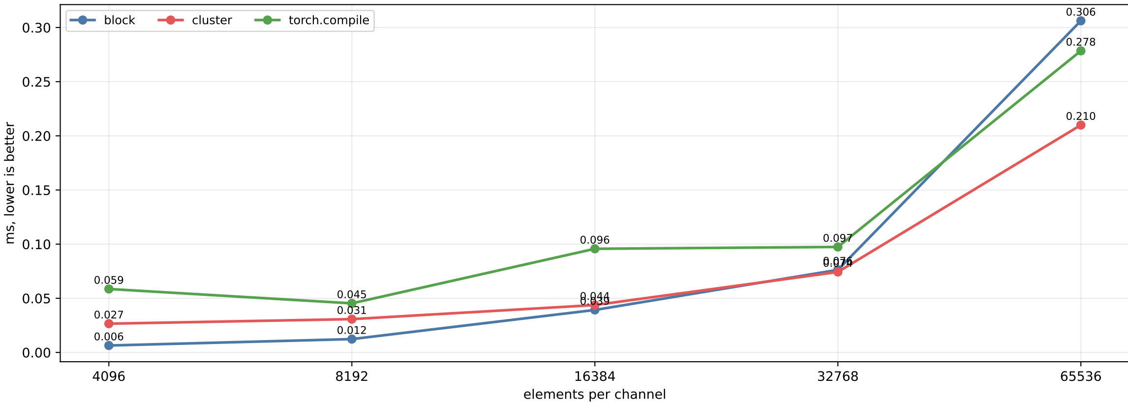
BatchNorm backward dx: ms, lower is better
