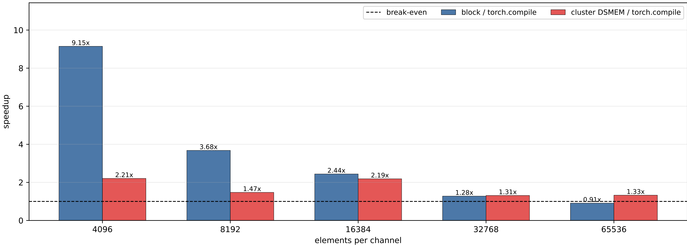
BatchNorm backward dx: speedup relative to torch.compile
