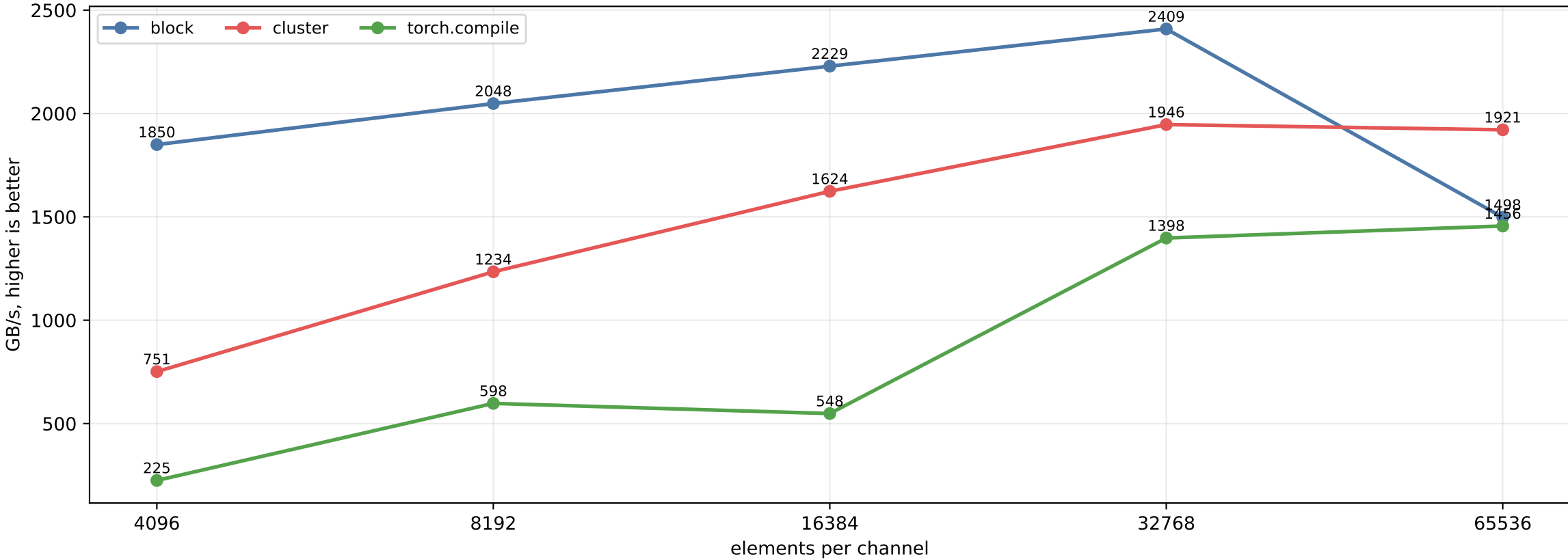
BatchNorm training forward: GB/s, higher is better
