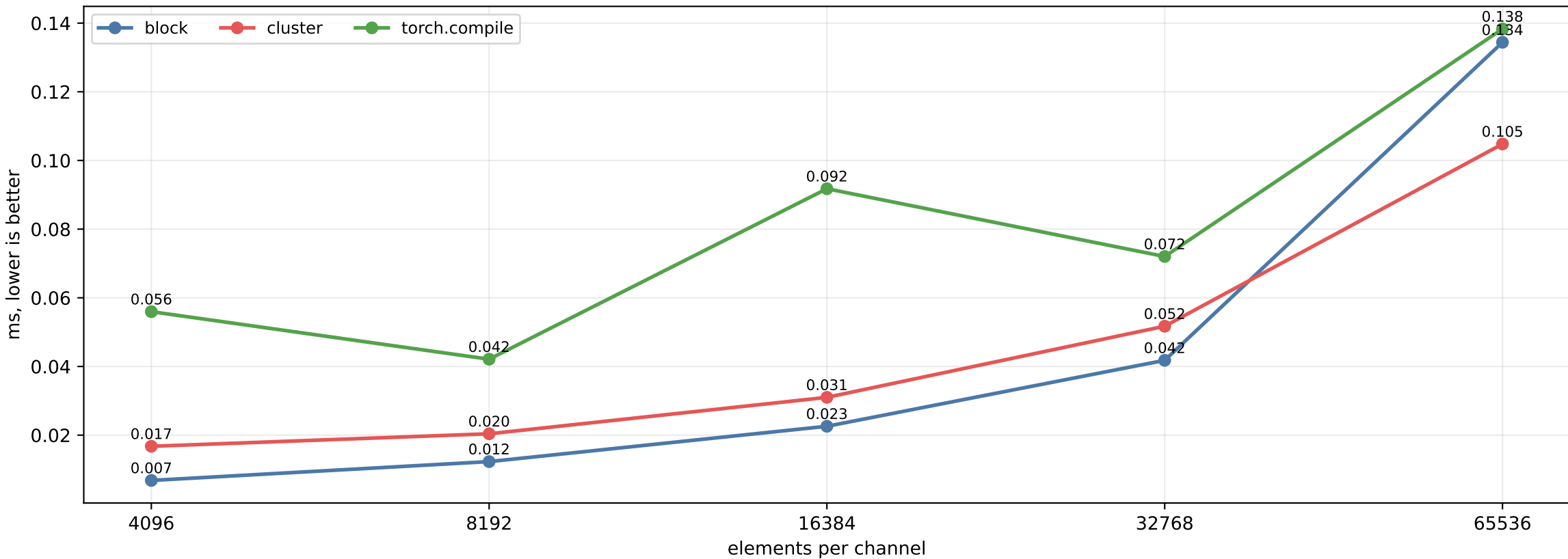
BatchNorm training forward: ms, lower is better
