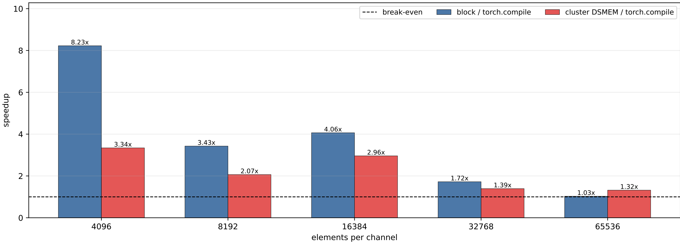
BatchNorm training forward: speedup relative to torch.compile
