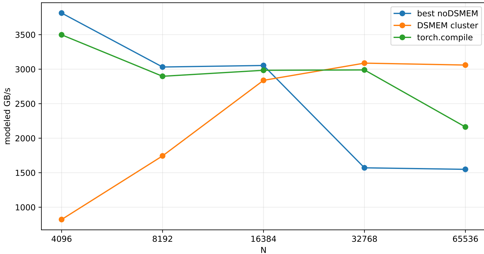
Cross-Entropy Backward Modeled Throughput
