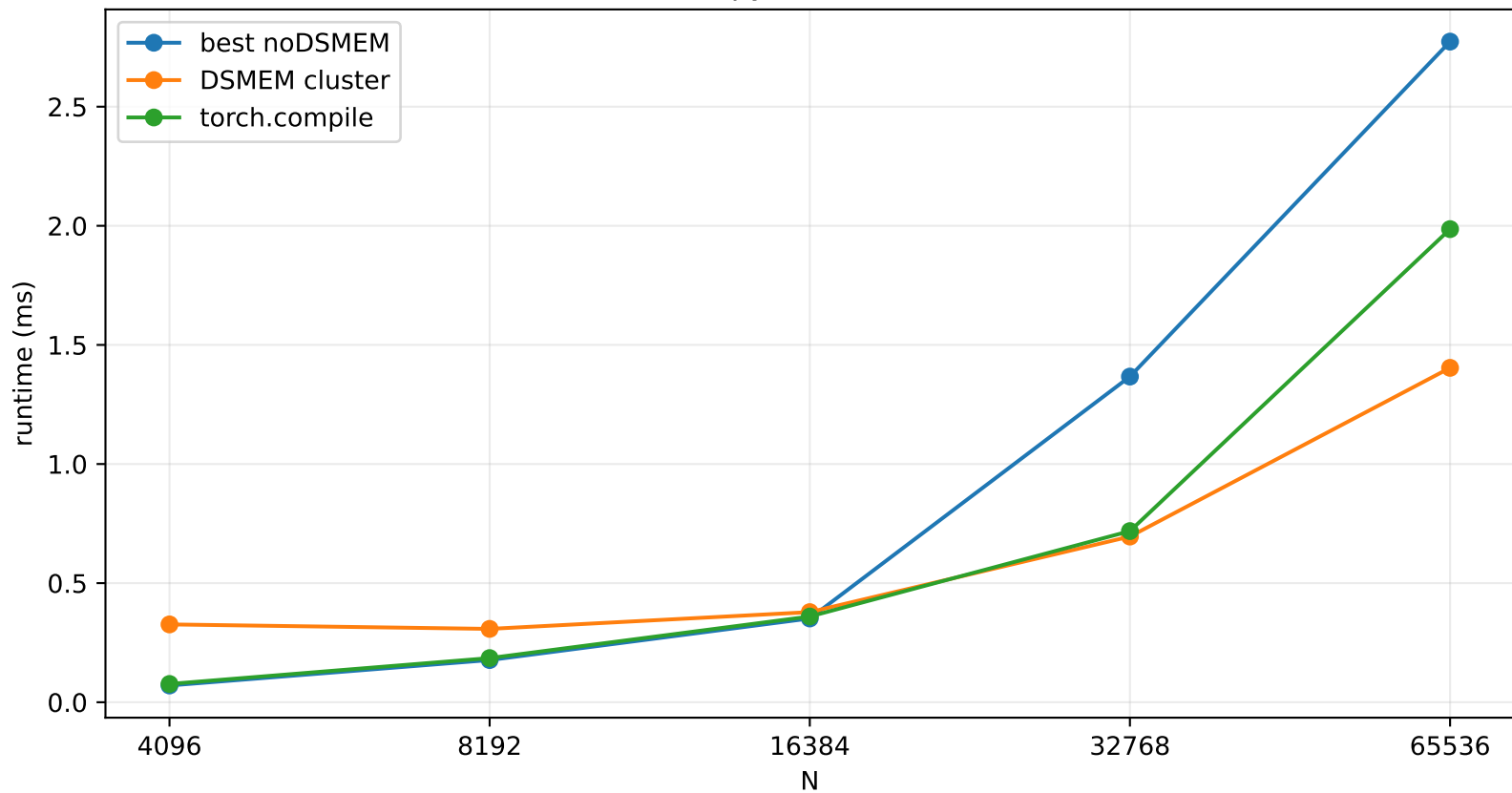
Cross-Entropy Backward Runtime
