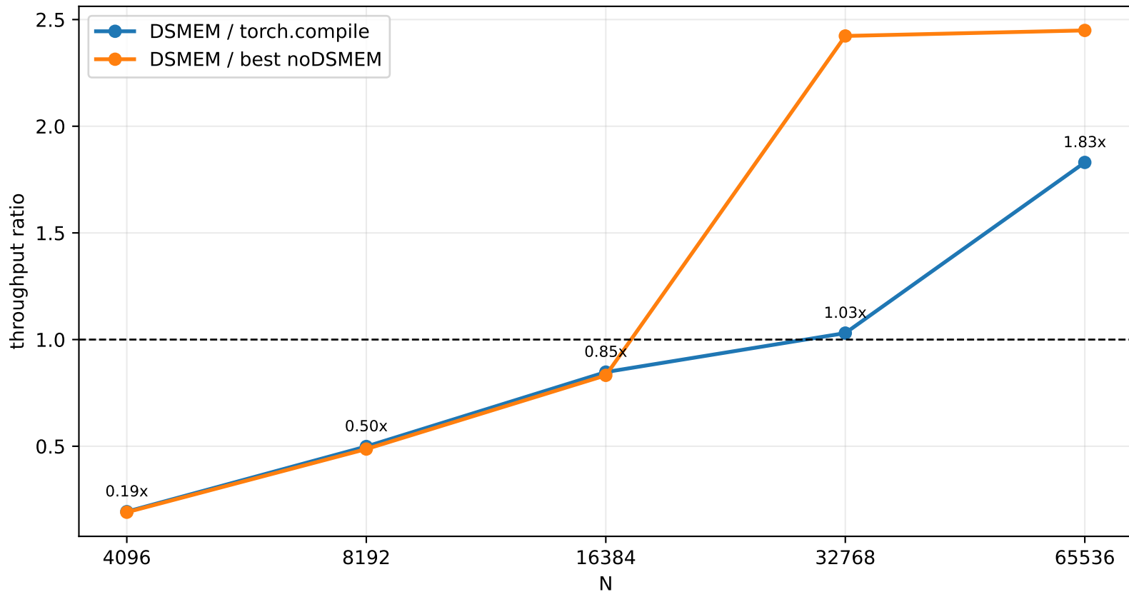
Entropy Backward DSMEM Speedup
