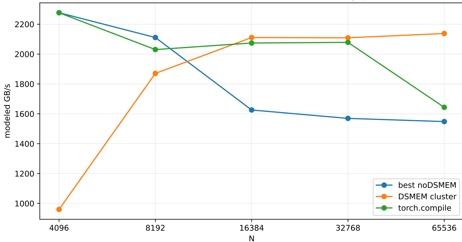
Row-wise Gated Standardization Modeled Throughput
