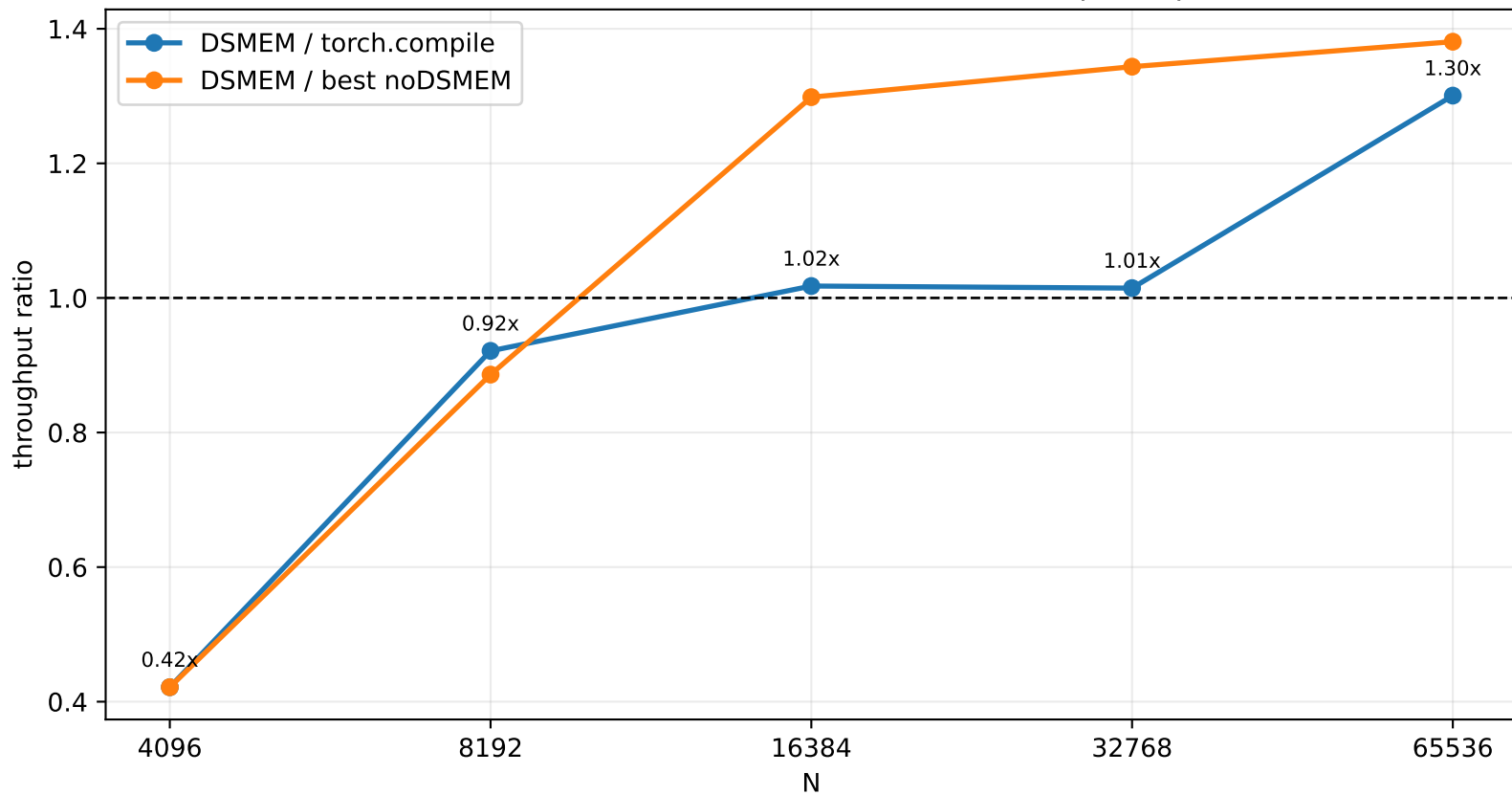
Row-wise Gated Standardization DSMEM Speedup
