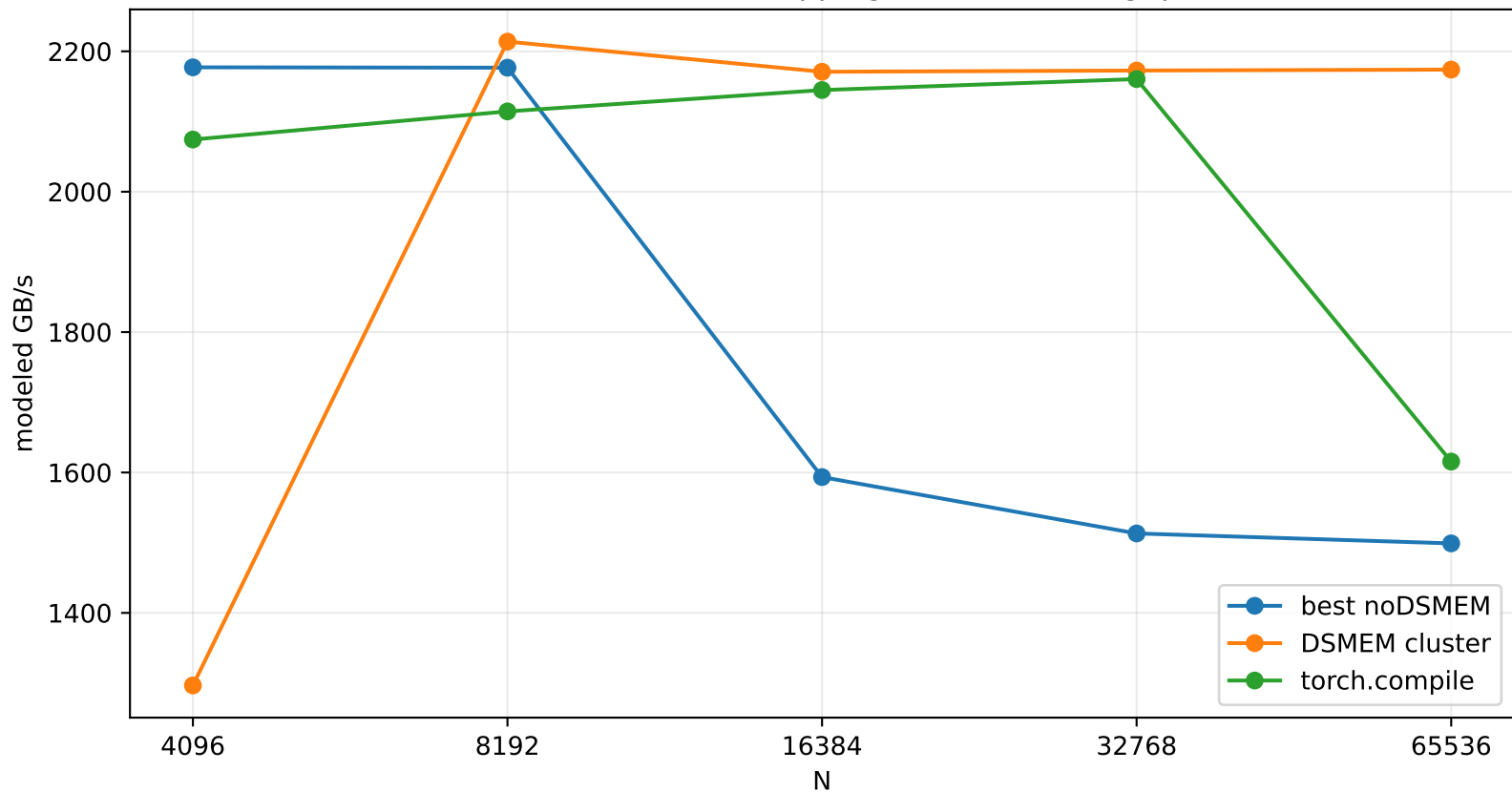
Gradient-Centralized Clipping Modeled Throughput
