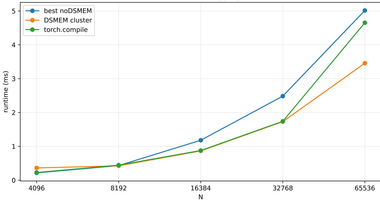
Gradient-Centralized Clipping Runtime
