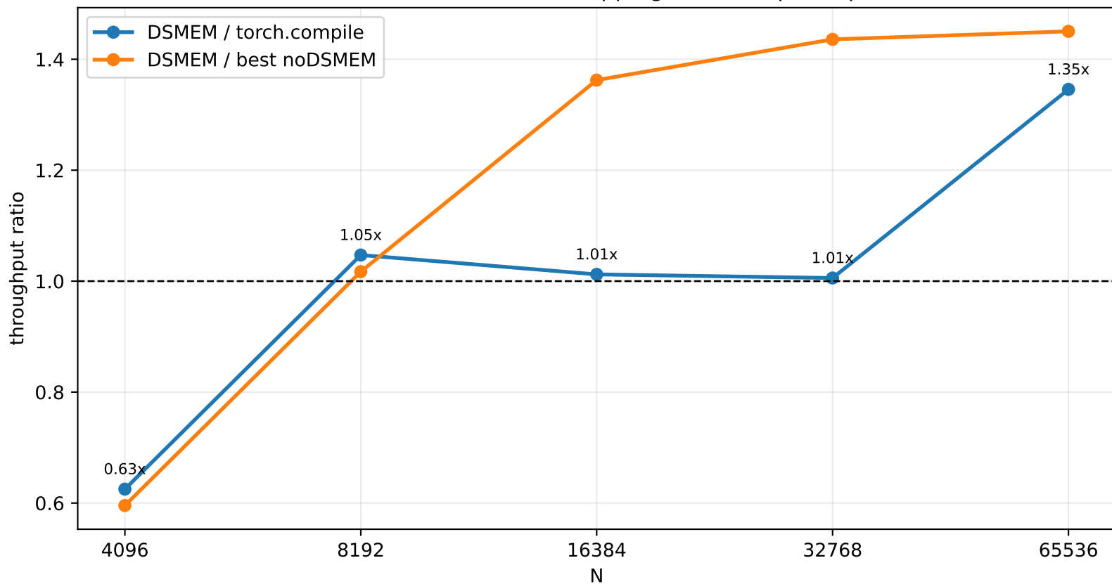
Gradient-Centralized Clipping DSMEM Speedup
