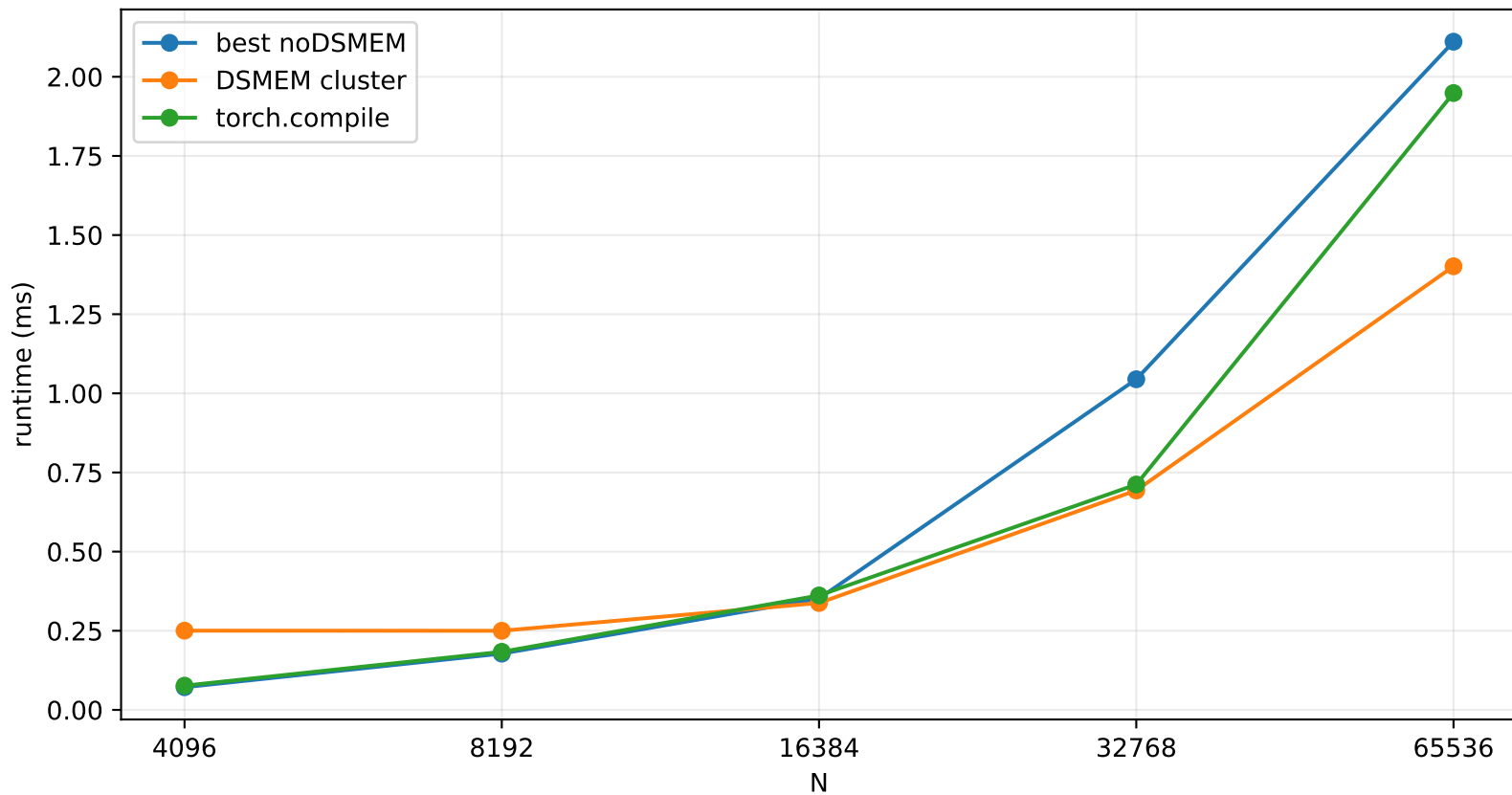
Row-wise L1 Normalization Runtime
