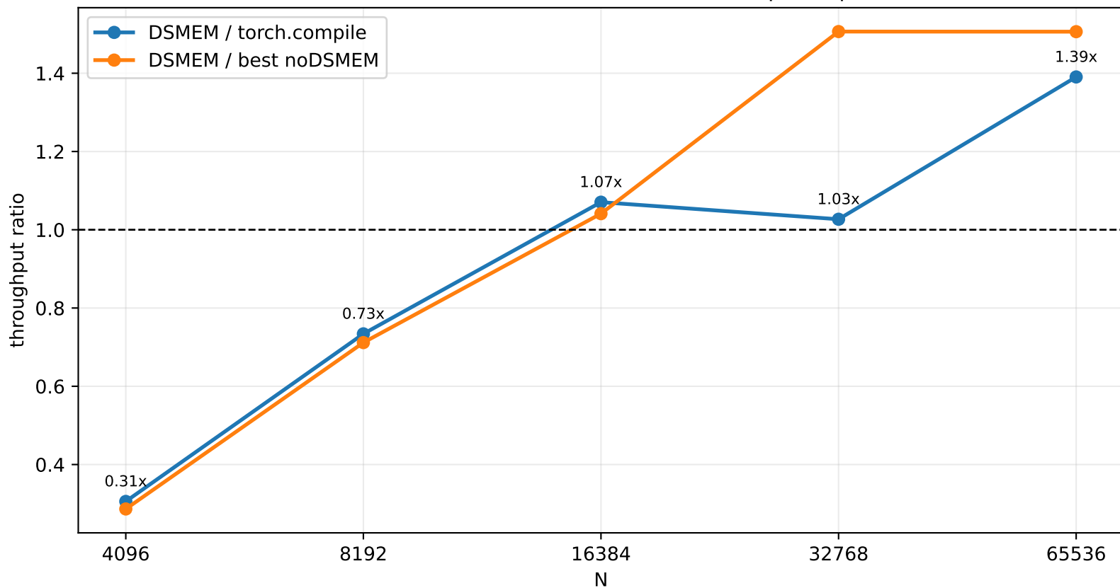
Row-wise L1 Normalization DSMEM Speedup
