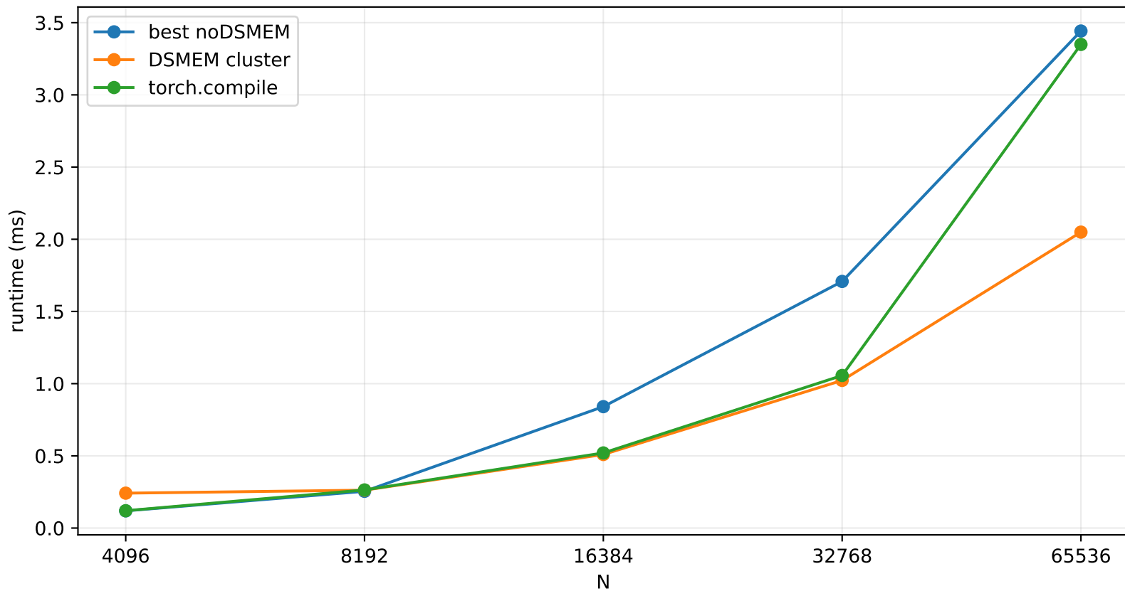
L2 Norm Backward Runtime
