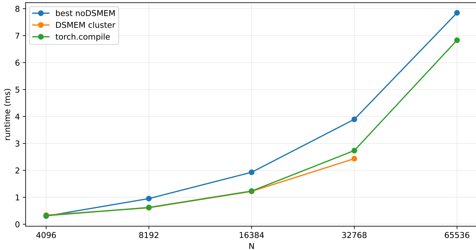
LAMB Trust-Ratio Runtime
