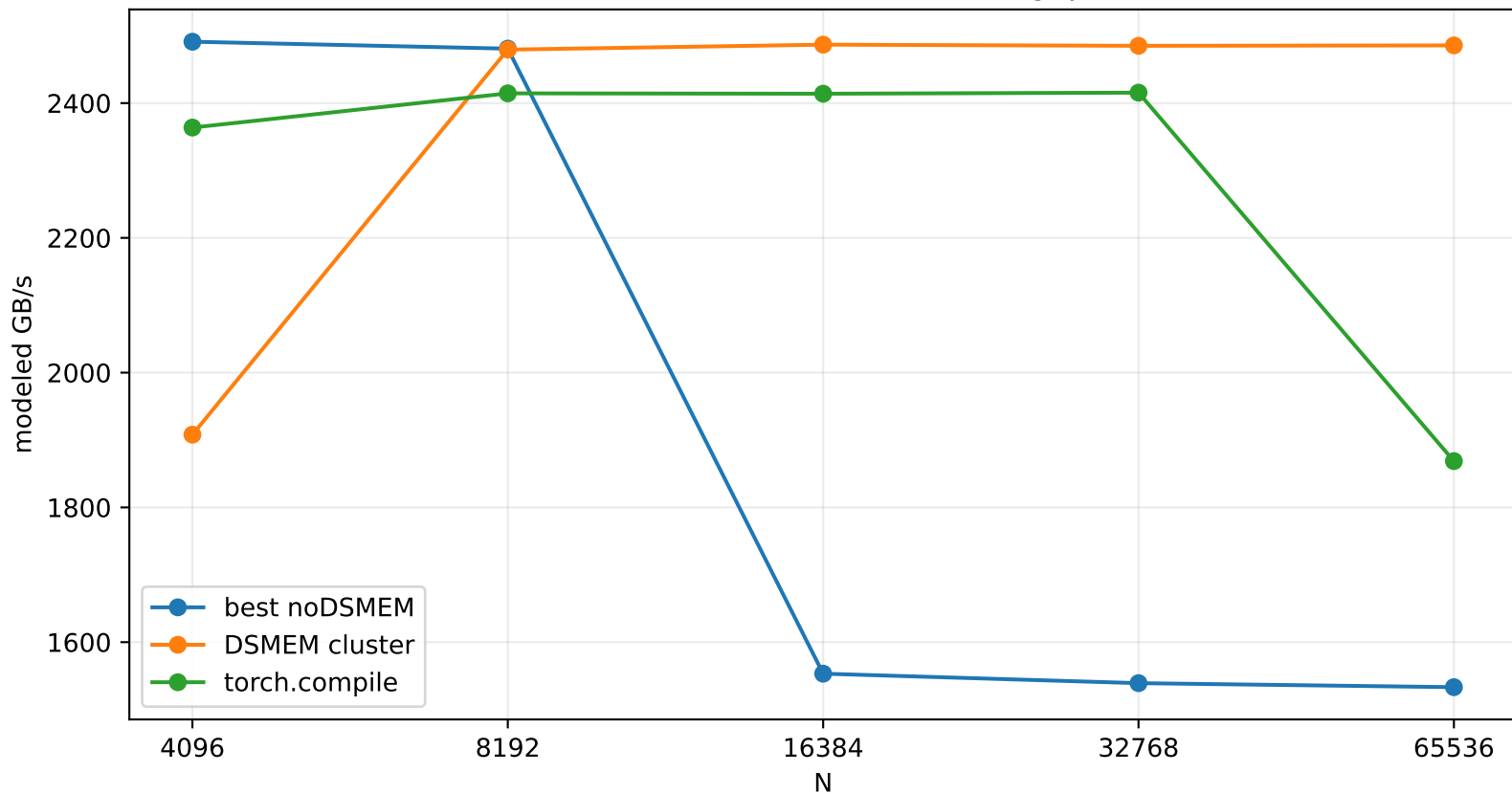
LARS Momentum Modeled Throughput
