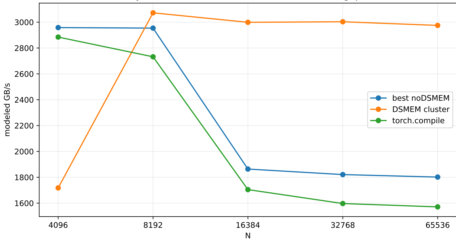
LayerNorm Affine Full Backward Modeled Throughput
