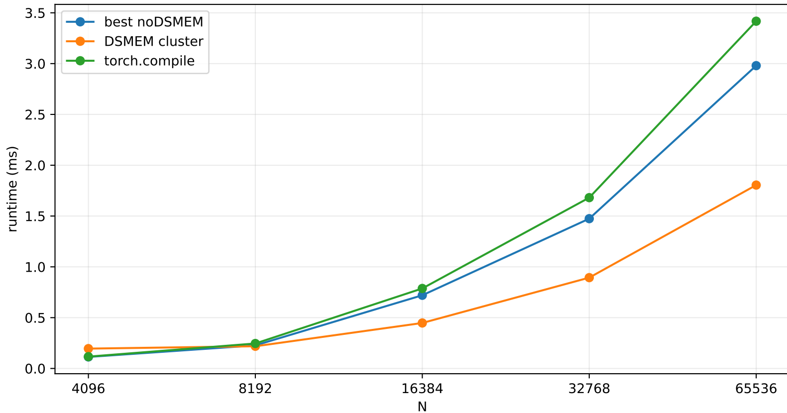
LayerNorm Affine Full Backward Runtime
