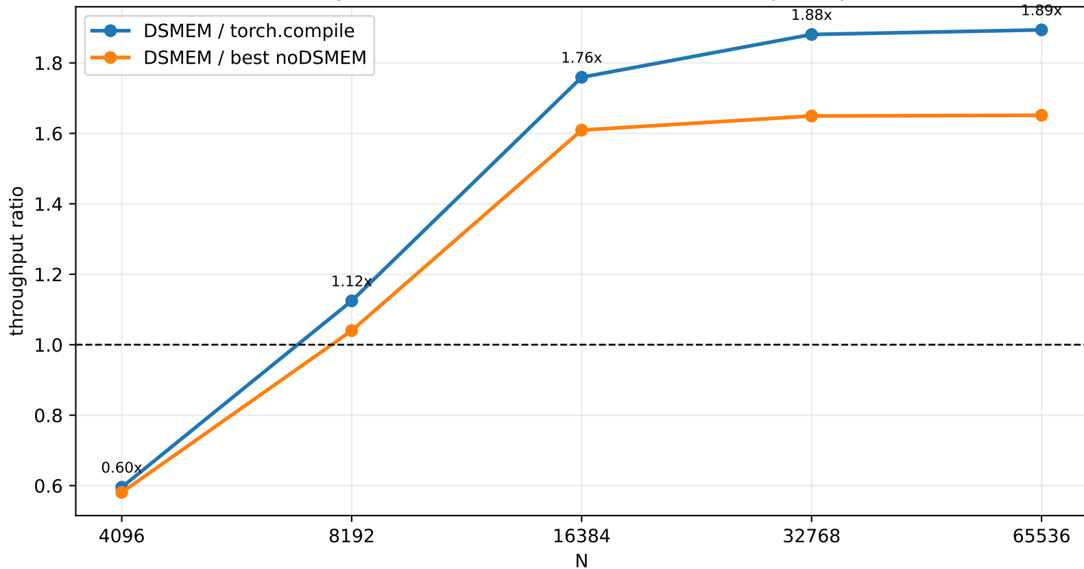
LayerNorm Affine Full Backward DSMEM Speedup
