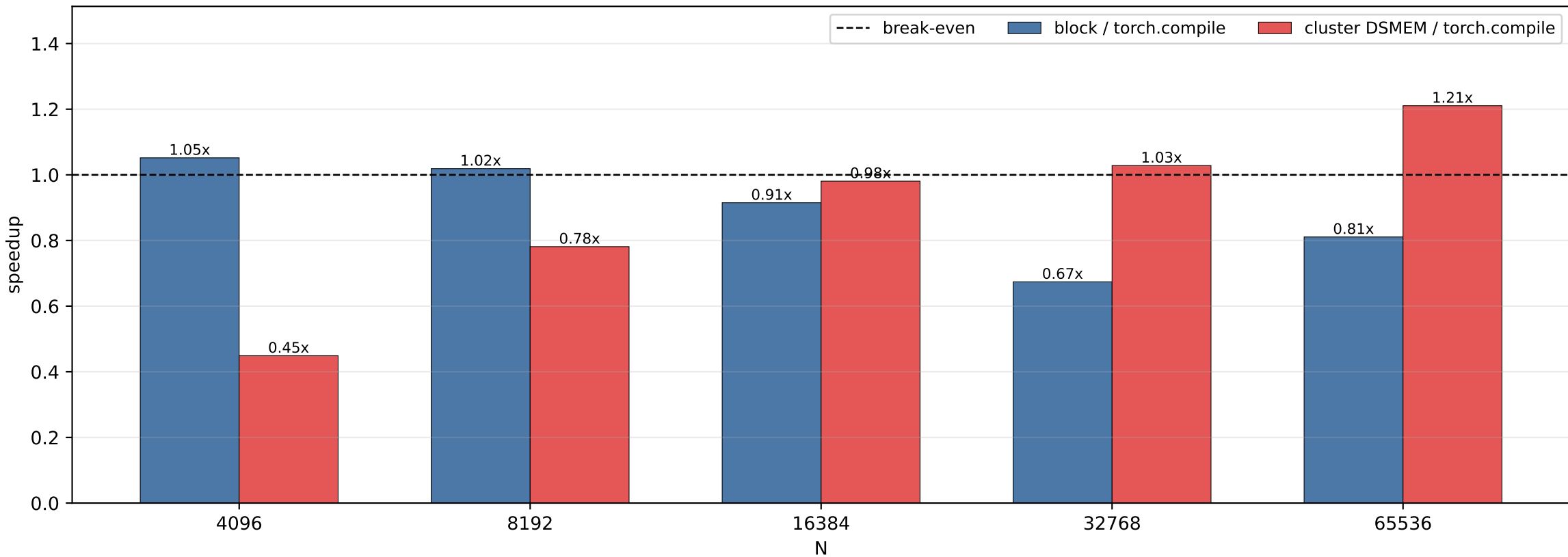
LayerNorm: speedup relative to torch.compile
