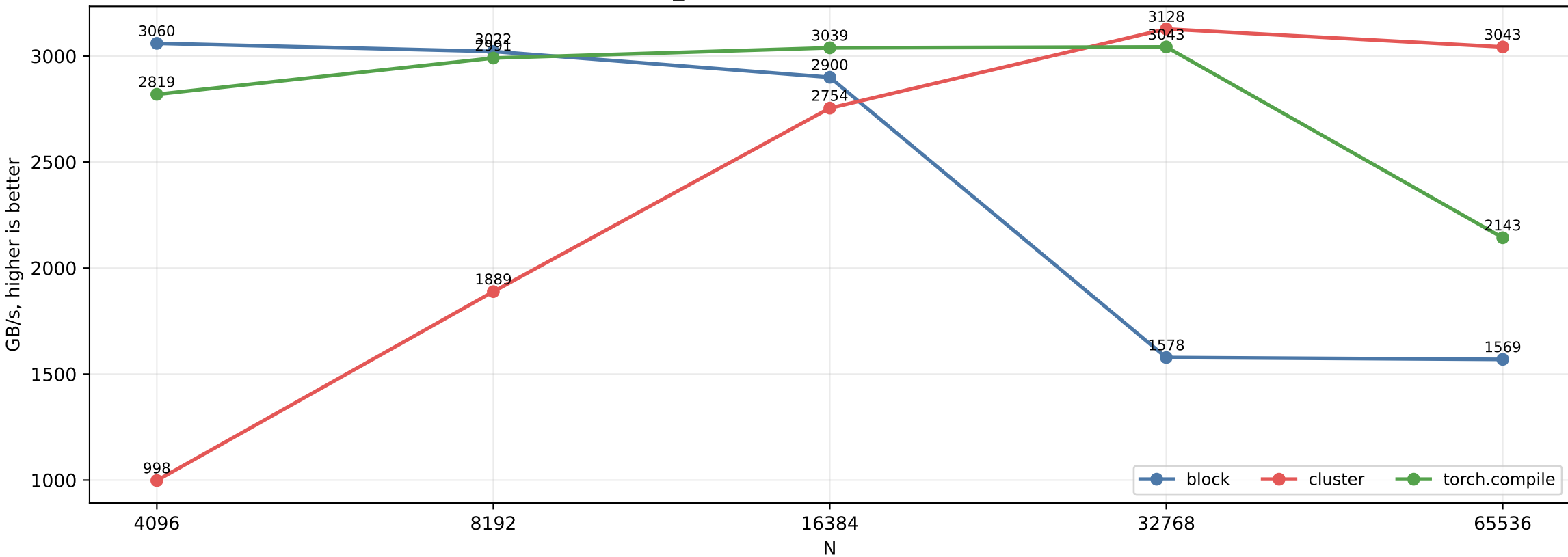
log_softmax: GB/s, higher is better
