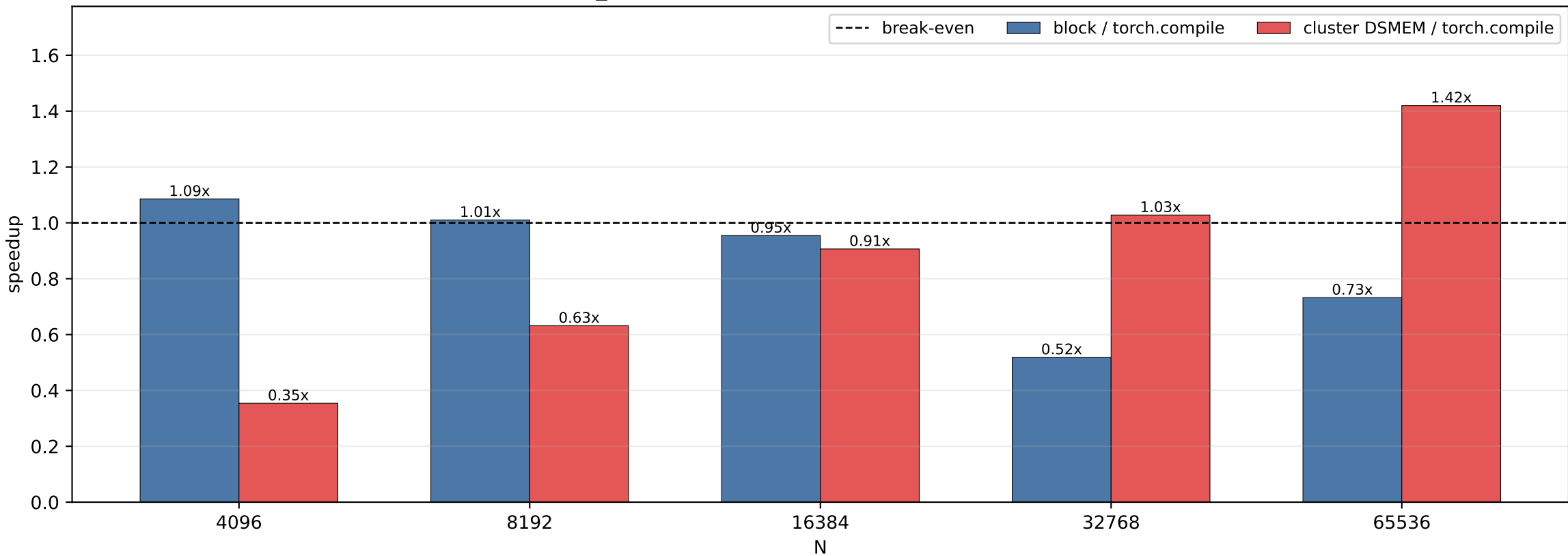
log_softmax: speedup relative to torch.compile
