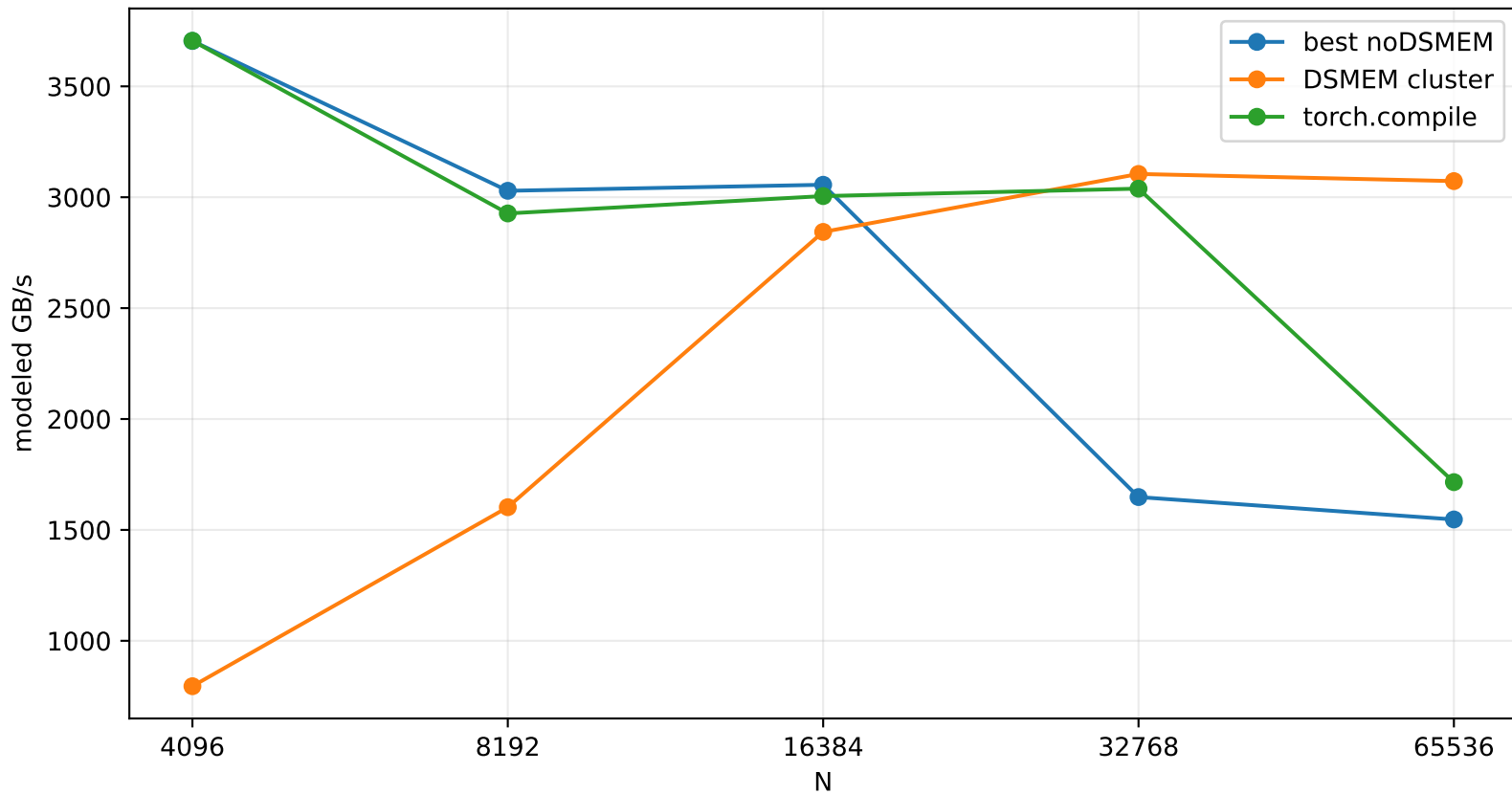
Row-wise MAD Normalization Modeled Throughput
