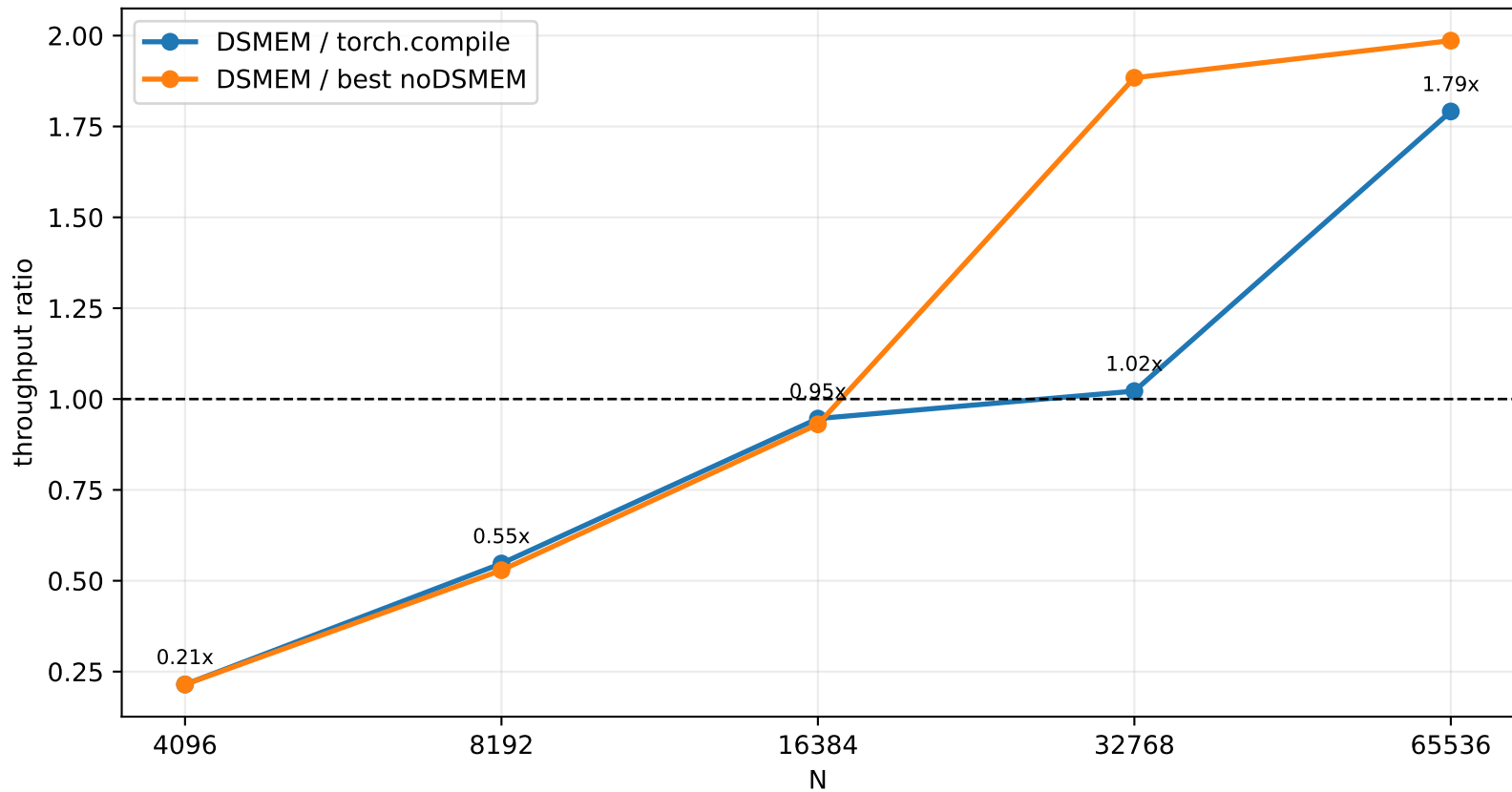
Row-wise MAD Normalization DSMEM Speedup
