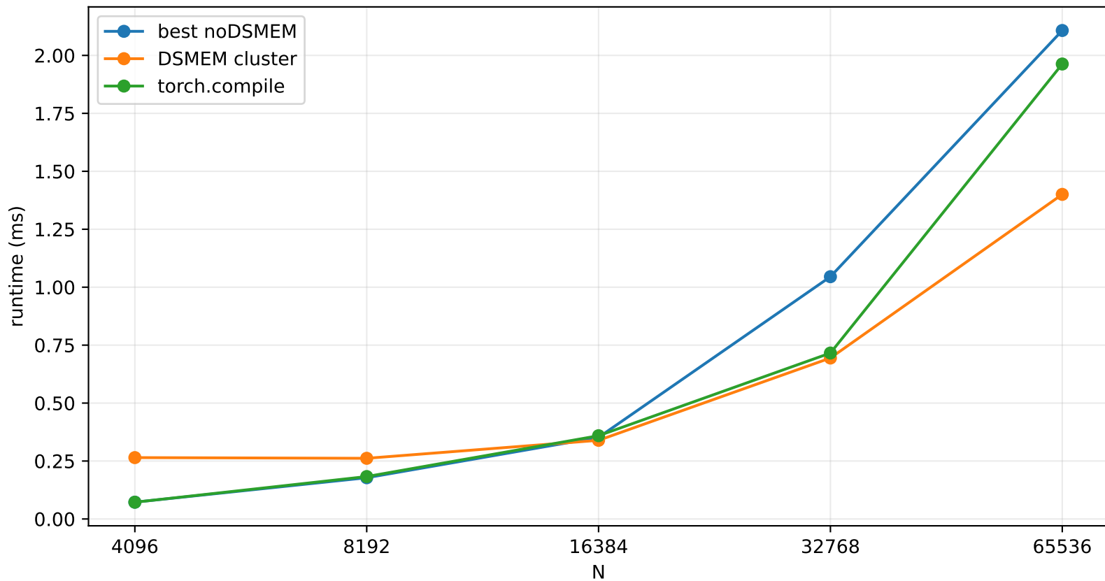
Row-wise Min-Max Normalization Runtime
