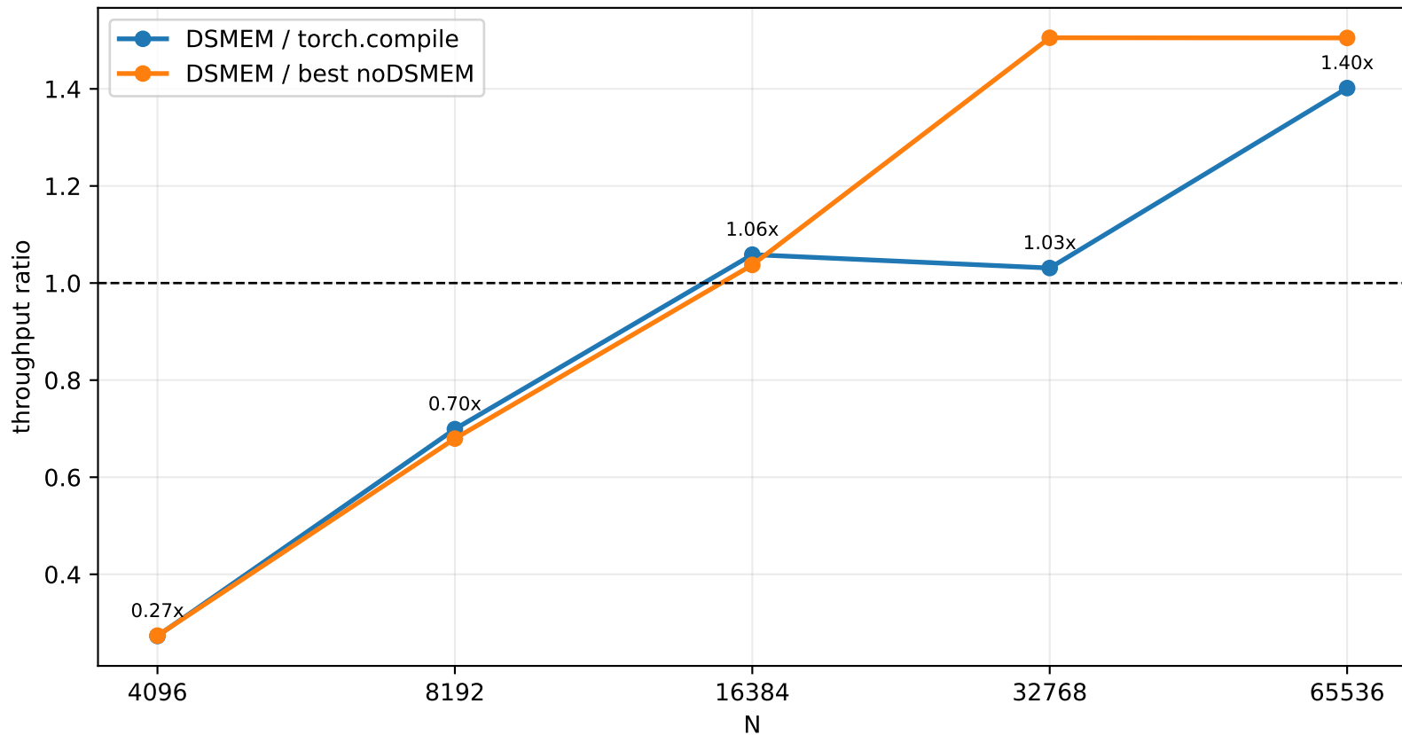
Row-wise Min-Max Normalization DSMEM Speedup
