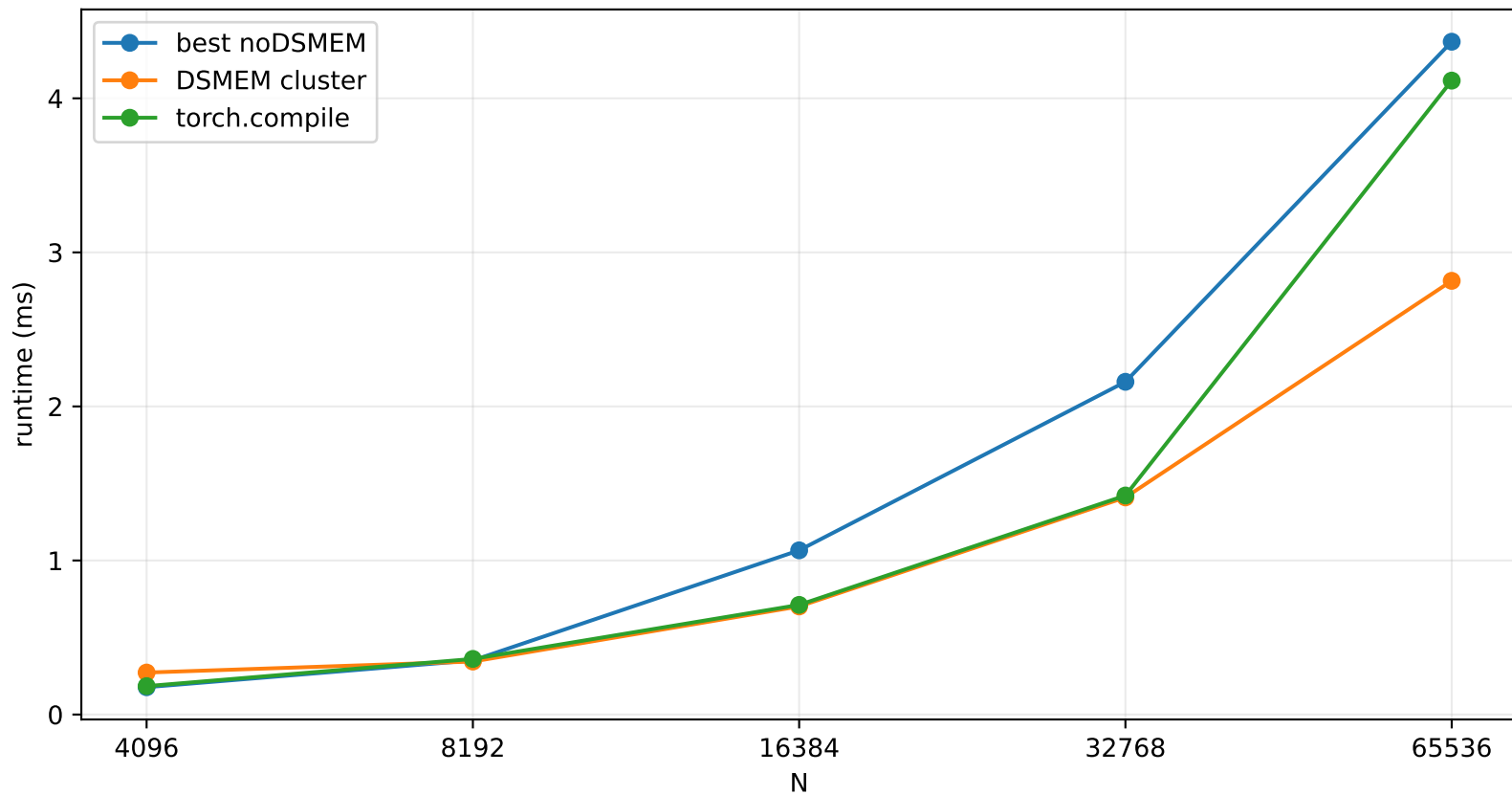
Pairwise Distance Backward Runtime
