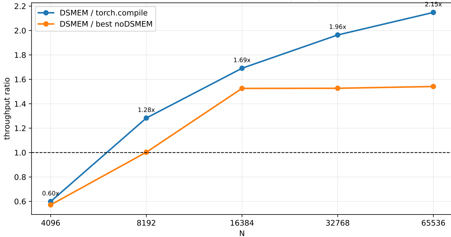
Pearson Backward DSMEM Speedup
