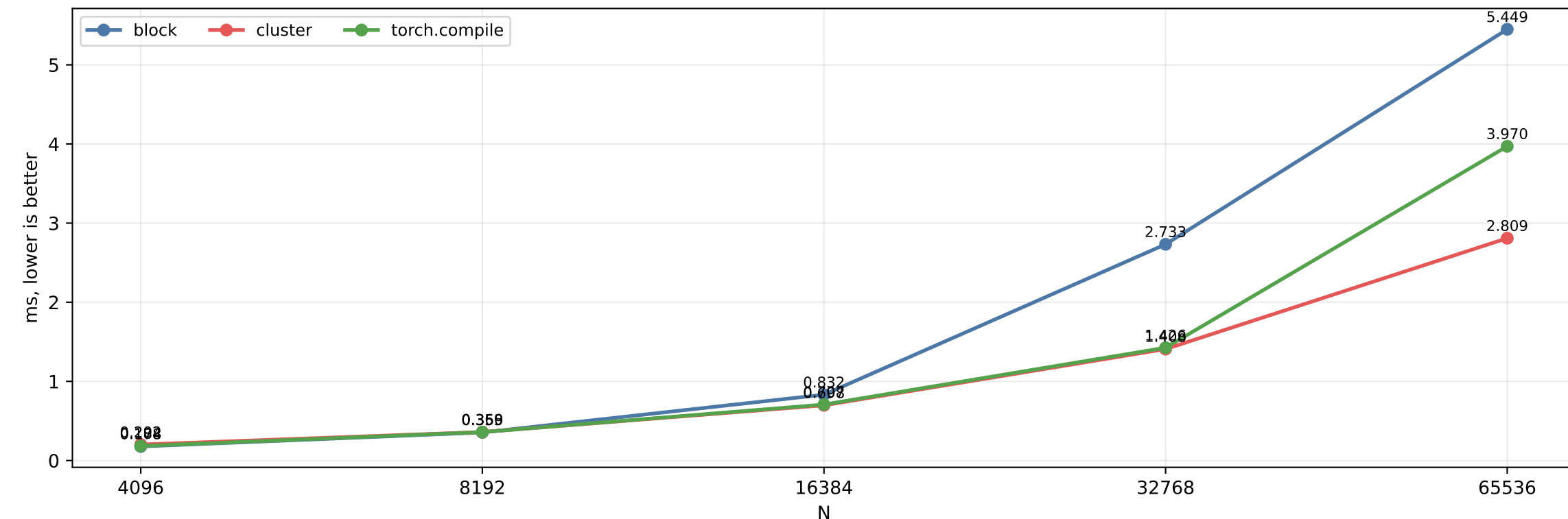
rmsnorm: runtime
