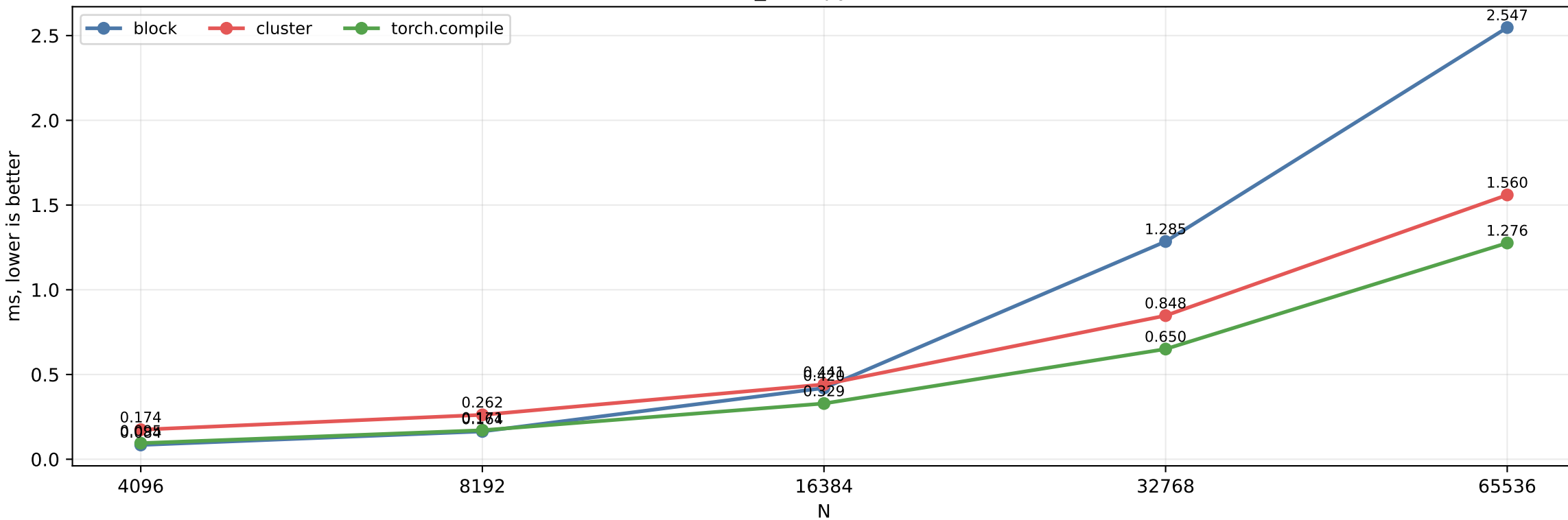
cross_entropy: runtime
