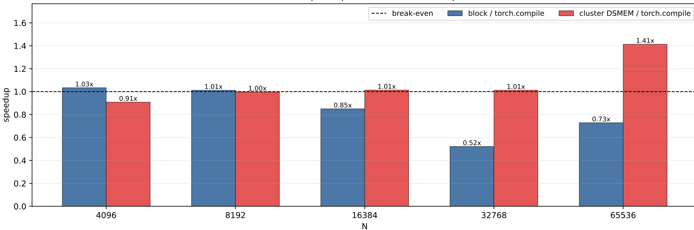
rmsnorm: speedup relative to torch.compile
