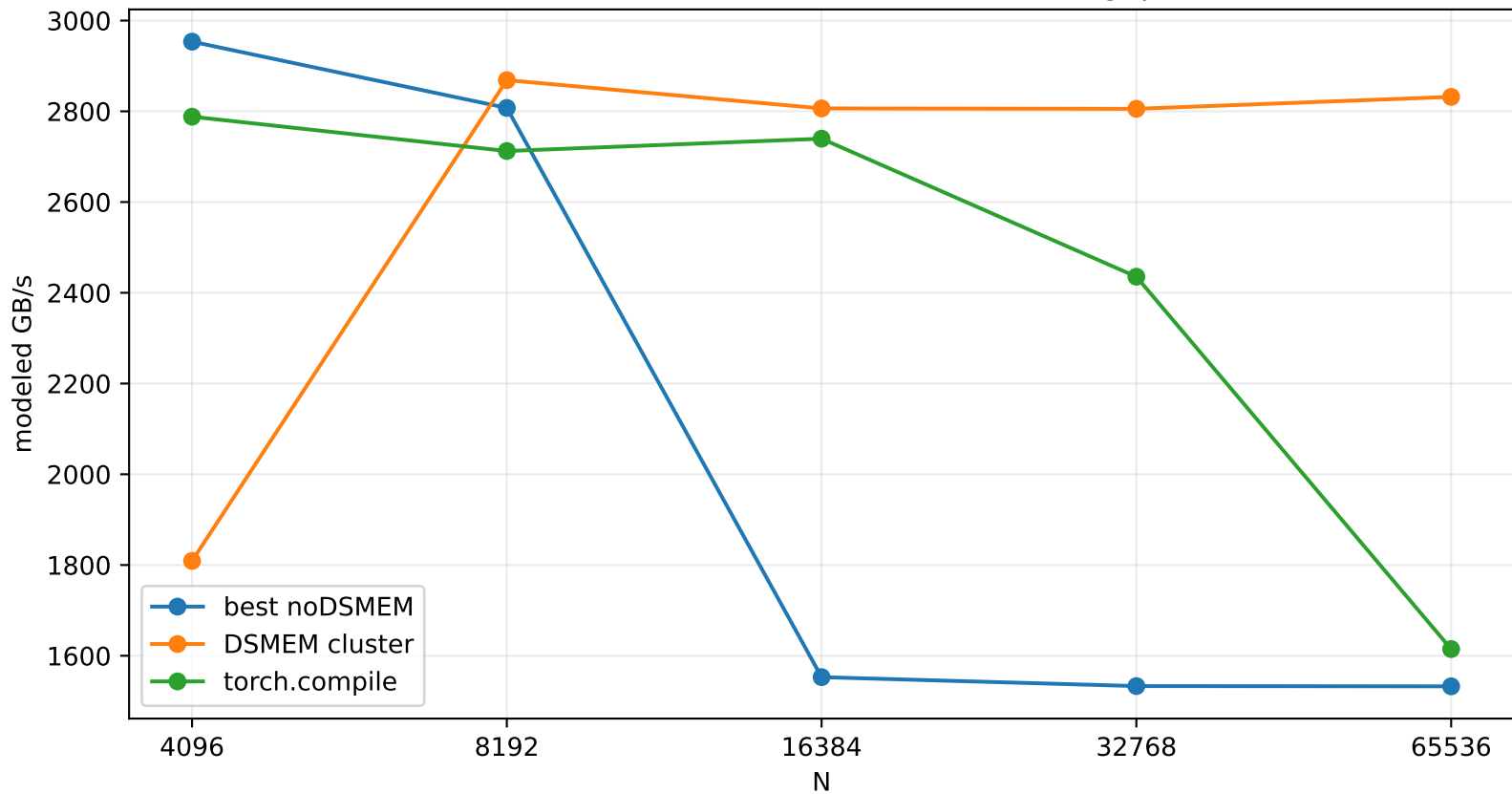
RMSNorm Gated Backward Modeled Throughput
