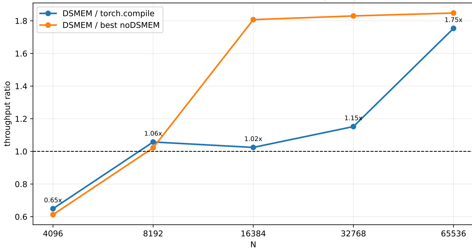
RMSNorm Gated Backward DSMEM Speedup
