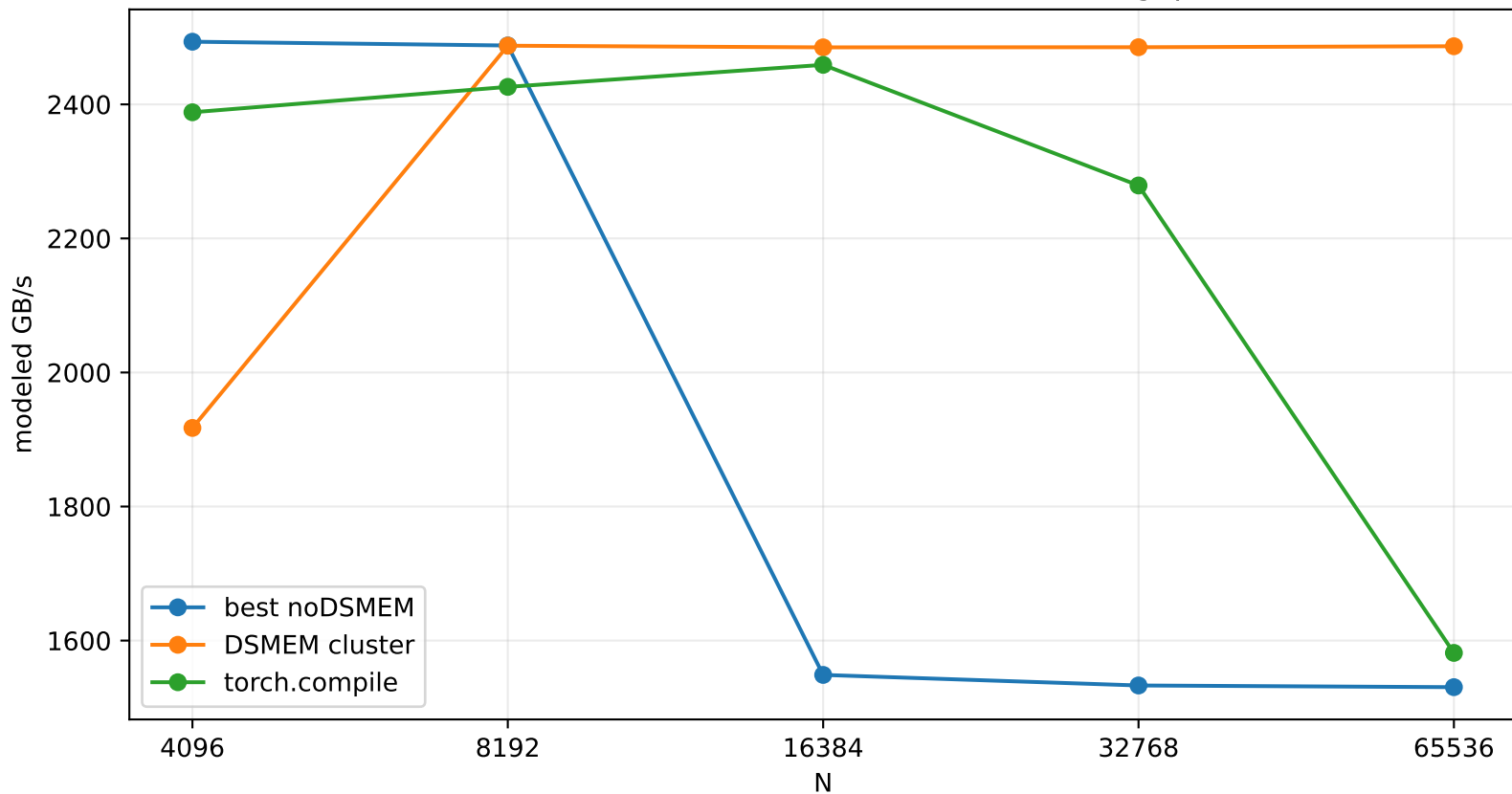
RMSNorm Gated Full Backward Modeled Throughput
