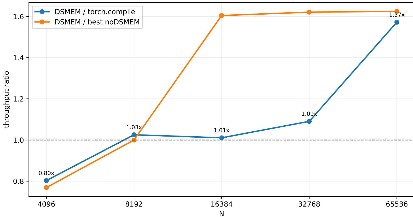
RMSNorm Gated Full Backward DSMEM Speedup
