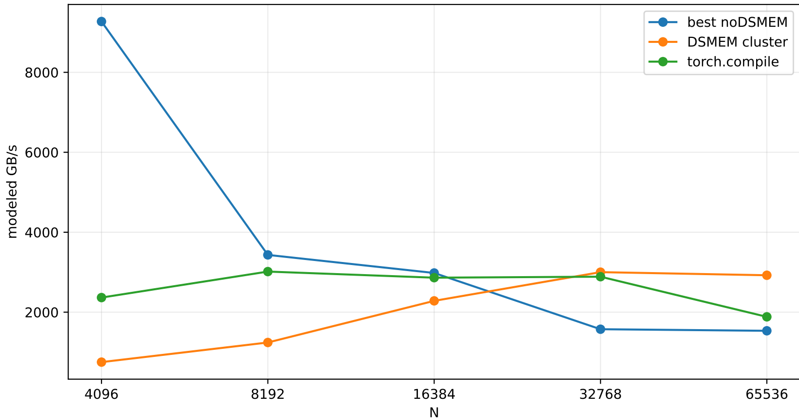
Row-wise Dynamic Quantization Modeled Throughput
